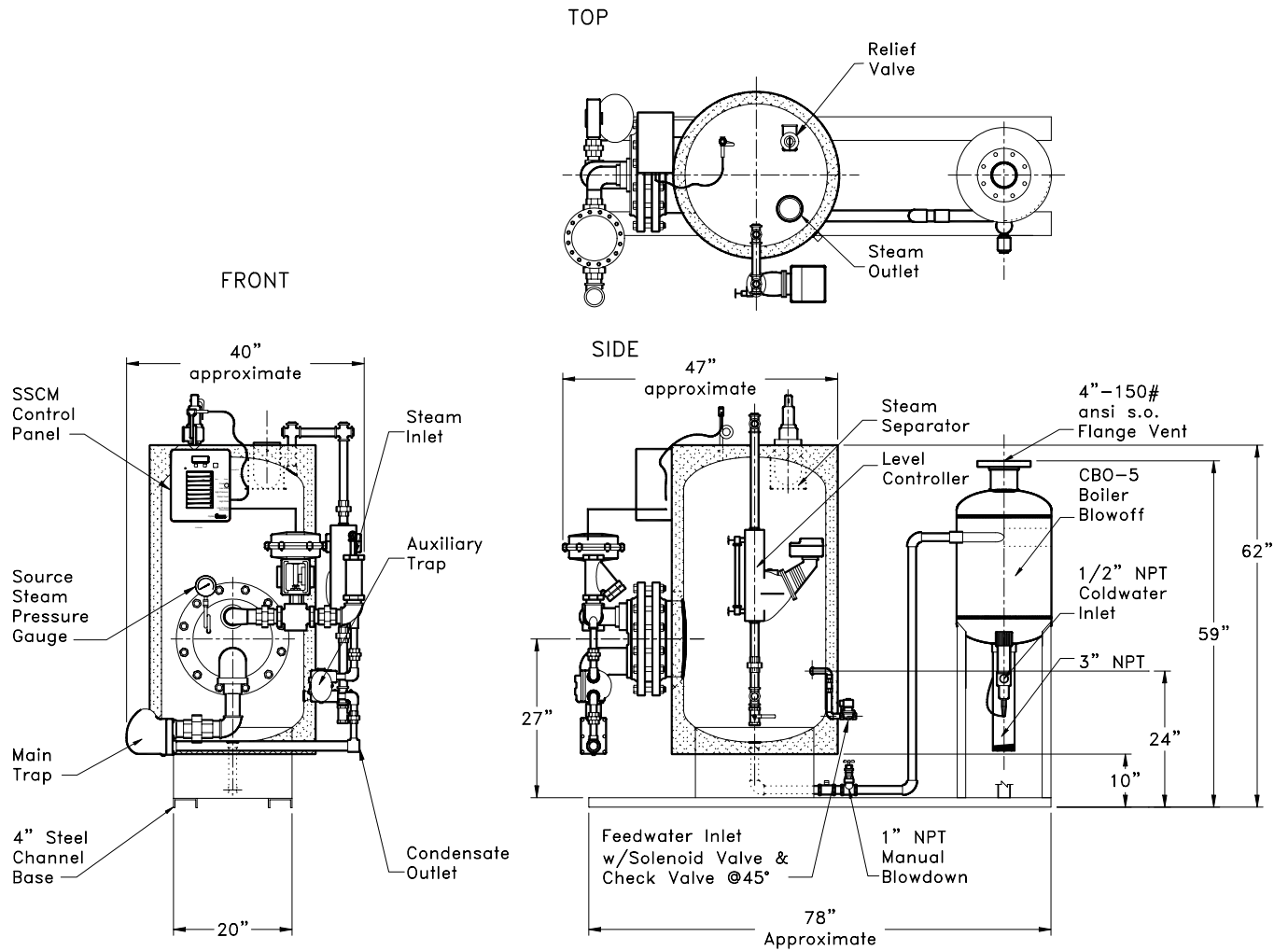
V90USG-CBO Energy Source - Steam
