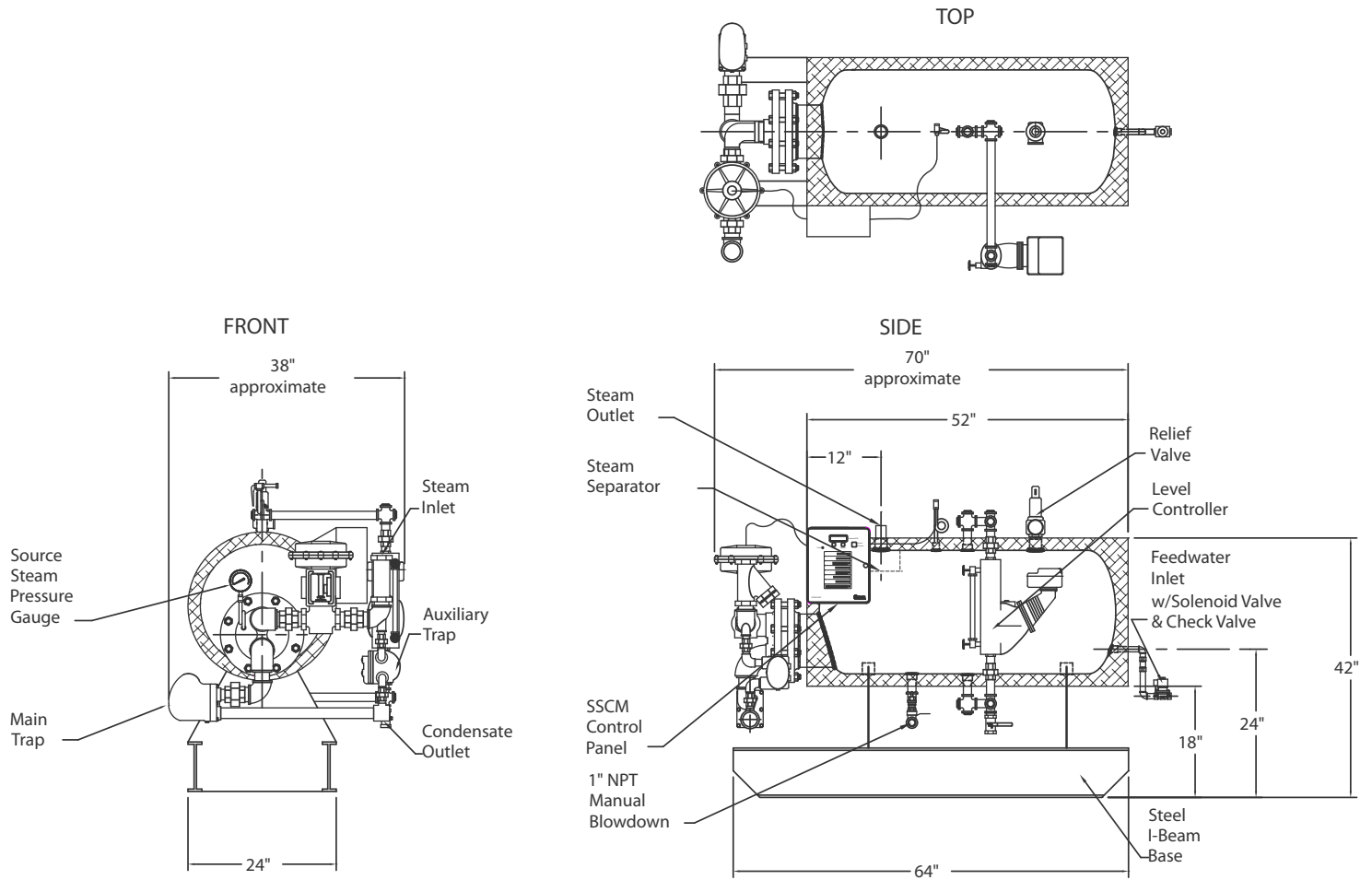
H60USG8XX Energy Source-Steam
