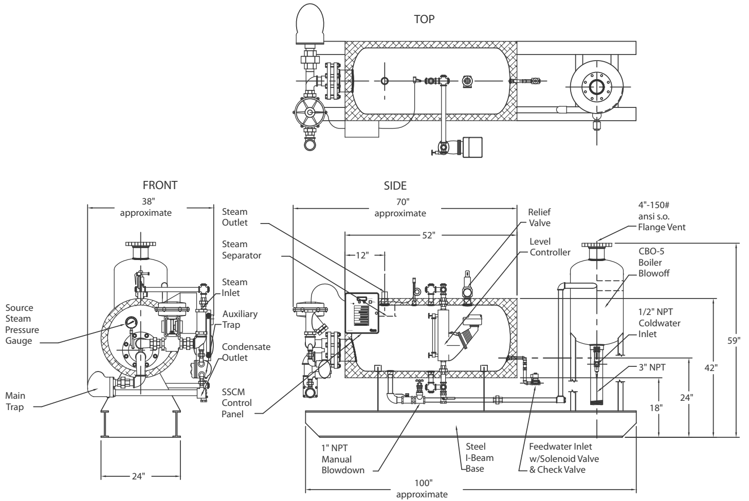
H60USG6XX-CBO Energy Source-Steam
