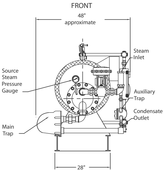
H120USG10XX Energy Source-Steam
