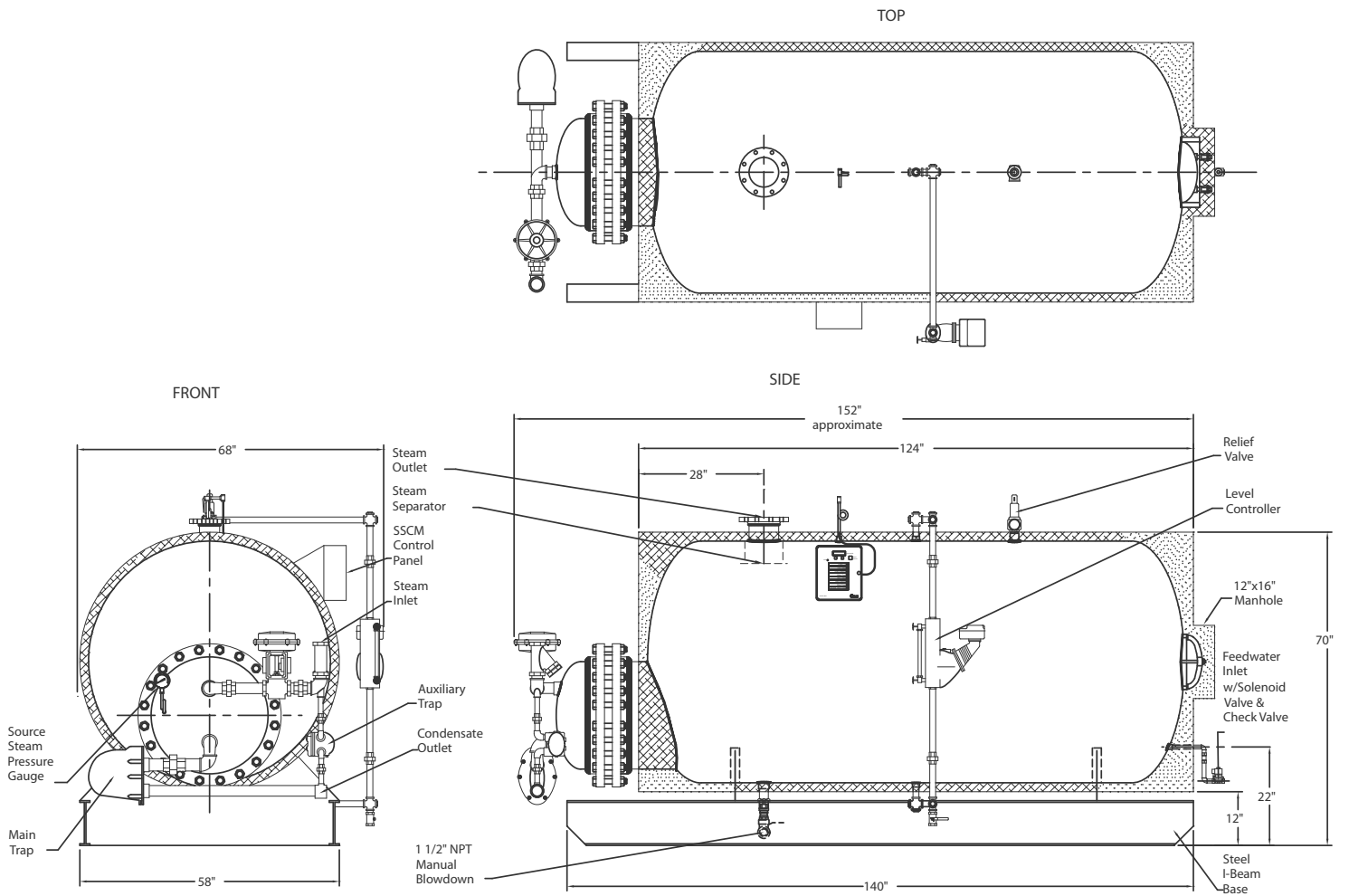
H1085USG24XX Energy Source-Steam
