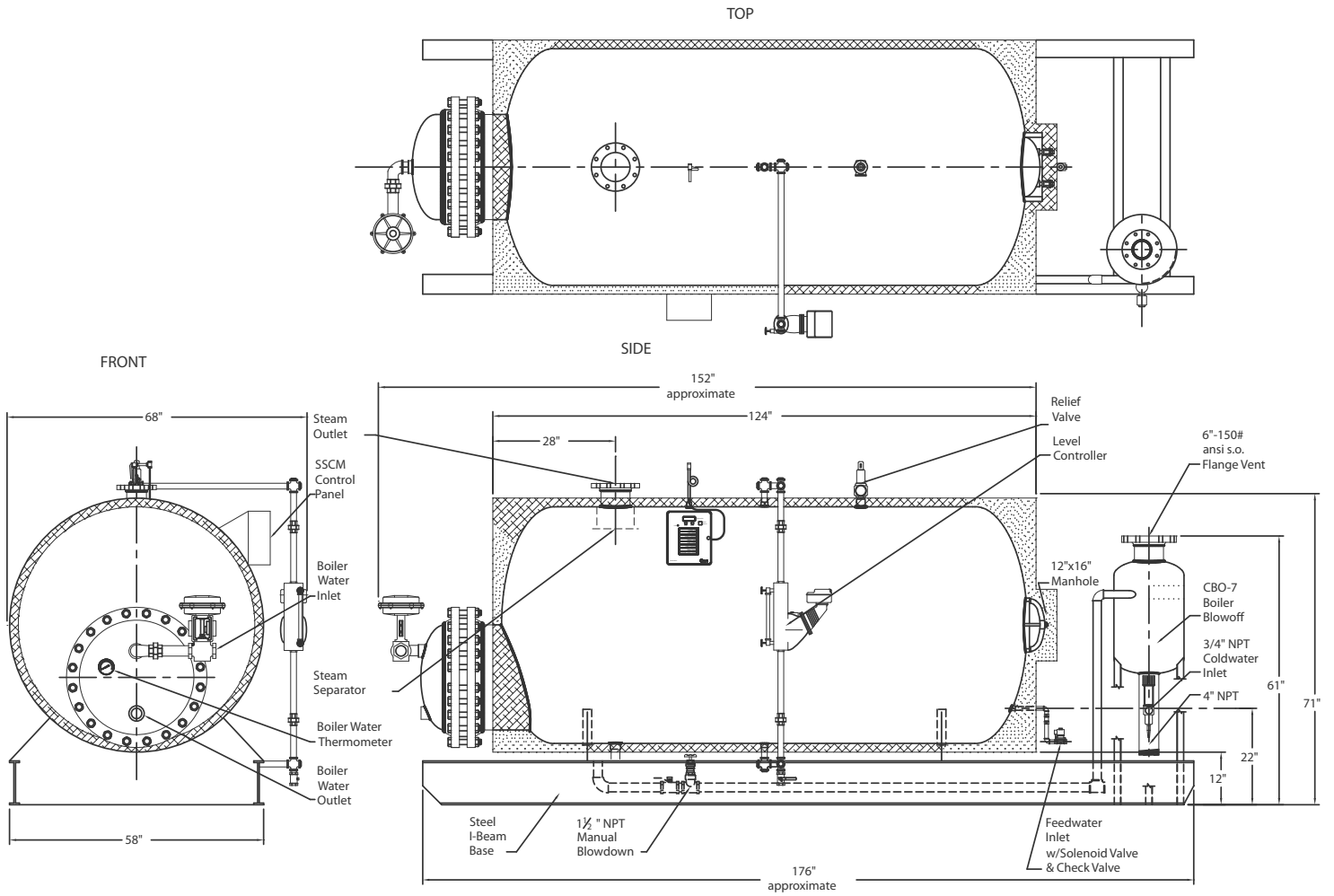
H1085USG24XX-W-CBO Energy Source-Boiler Water
